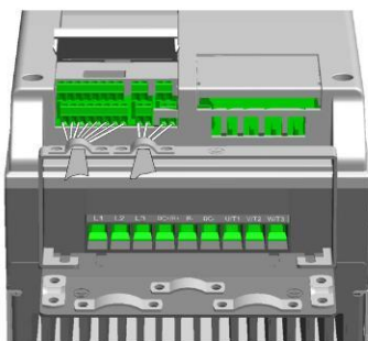
Figure 17: Install the control cables (MI4 - MI15)
