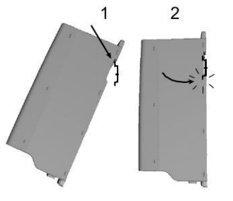
Figure 3: DIN rail mounting, MI1 - MI3
